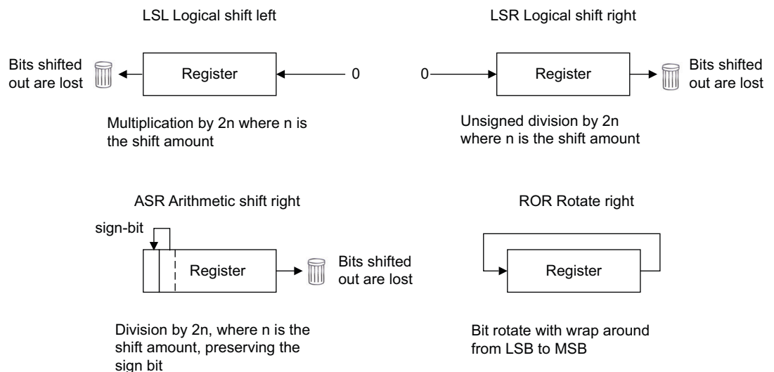
Figure 6-1 Shift operations
